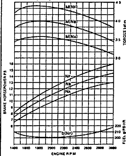
D750-B (DIN)
